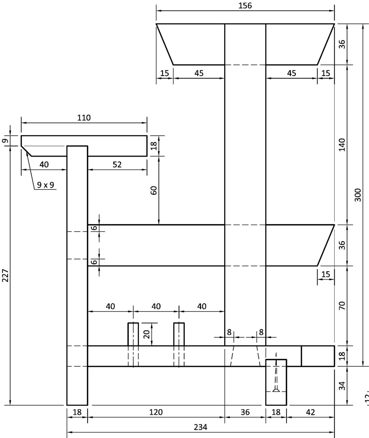
Elevation/Aghaidhchló
